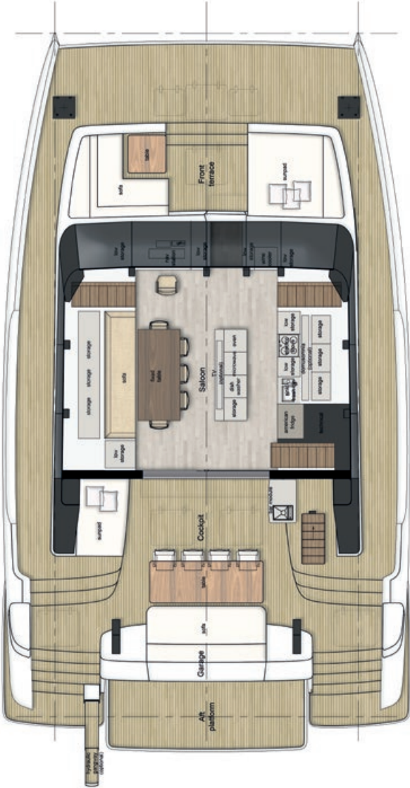
MAIN DECK
